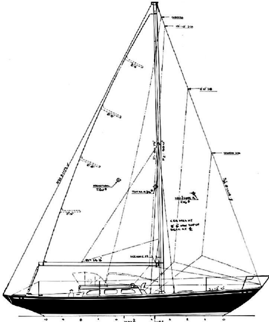
Sail Plan
